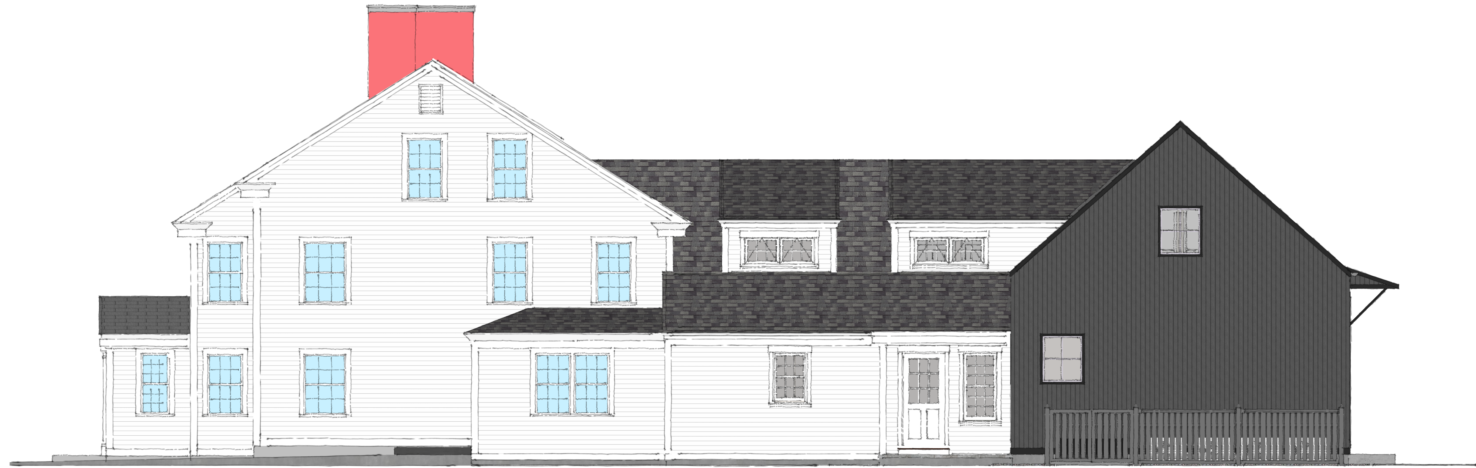
EAST ELEVATION
